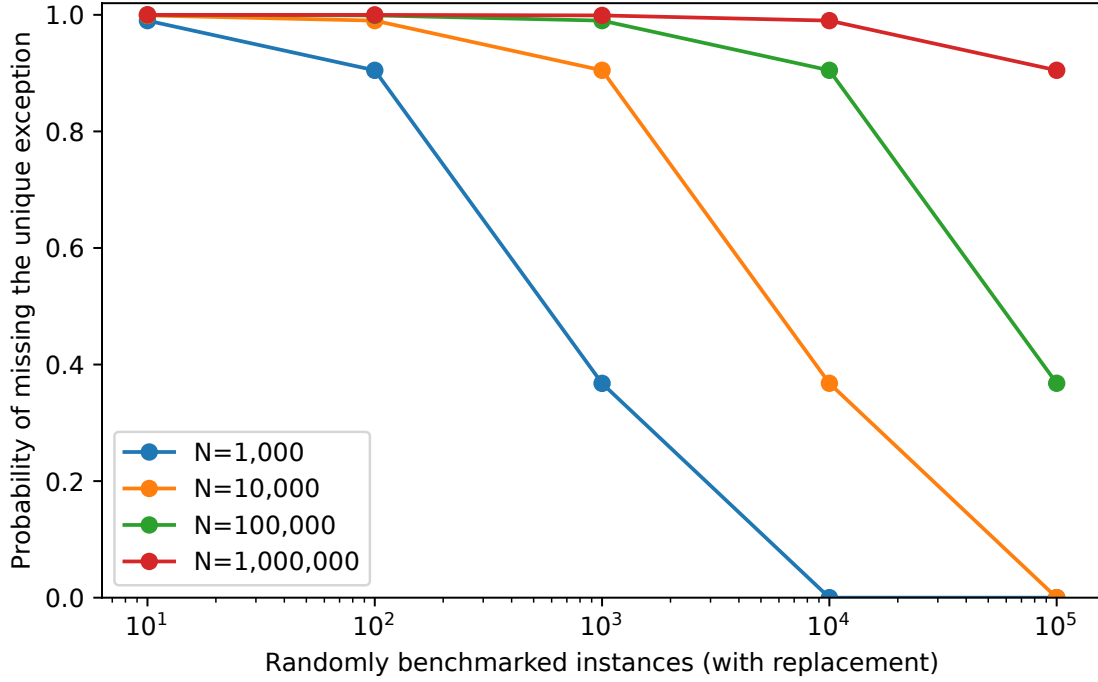
Figure 5: A high benchmark success rate cannot certify a universal theorem. When one exceptional instance is hidden among N , random testing can miss it with high probability even for large test budgets.
